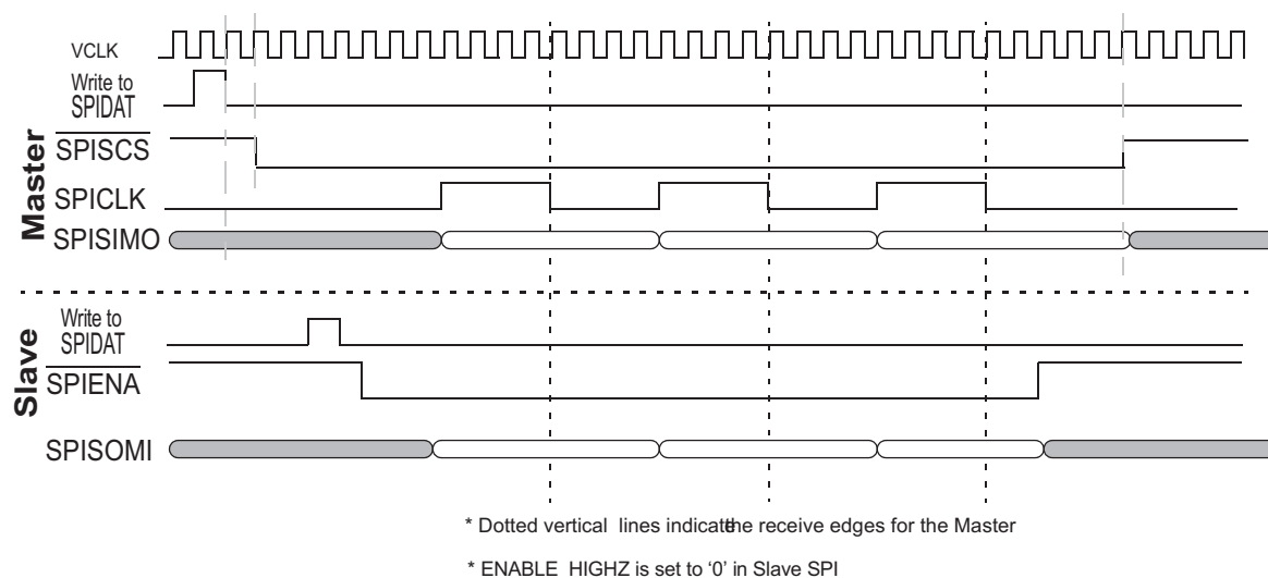
Figure 21-70. SPI/MibSPI Pins During Master/Slave Mode with 5-pin Configuration
