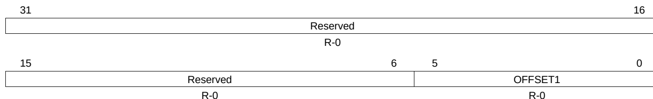
Figure 17-38. Offset Index Priority Level 1 Register (HETOFF1) [offset = 0Ch]
