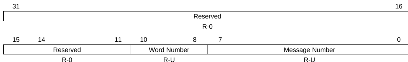
Figure 20-25. Parity Error Code Register (DCAN PERR) [offset = 1Ch]
