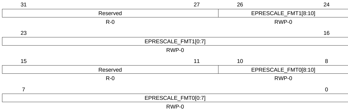
Figure 21-60. SPI Extended Prescale Register 1 (EXTENDED_PRESCALE1 for SPIFMT0 and SPIFMT1) [offset = 138h]
