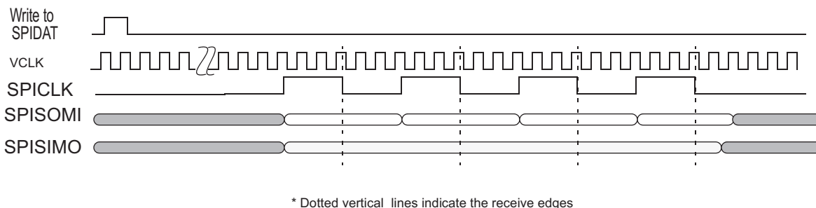
Figure 21-71. SPI/MibSPI Pins During Slave Mode 3-pin Configuration
