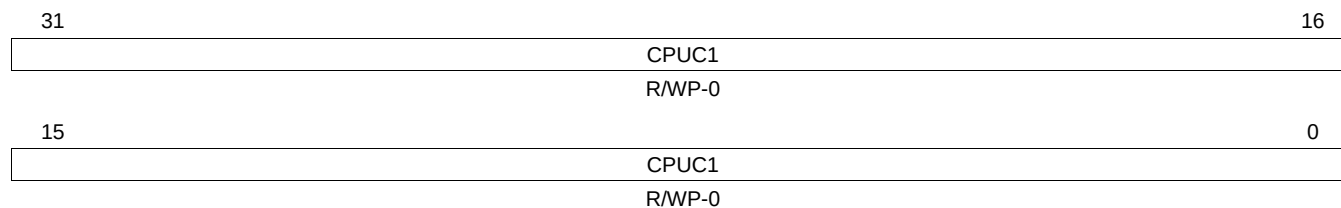
Figure 12-18. RTI Compare Up Counter 1 Register (RTICPUC1) [offset = 38h]
