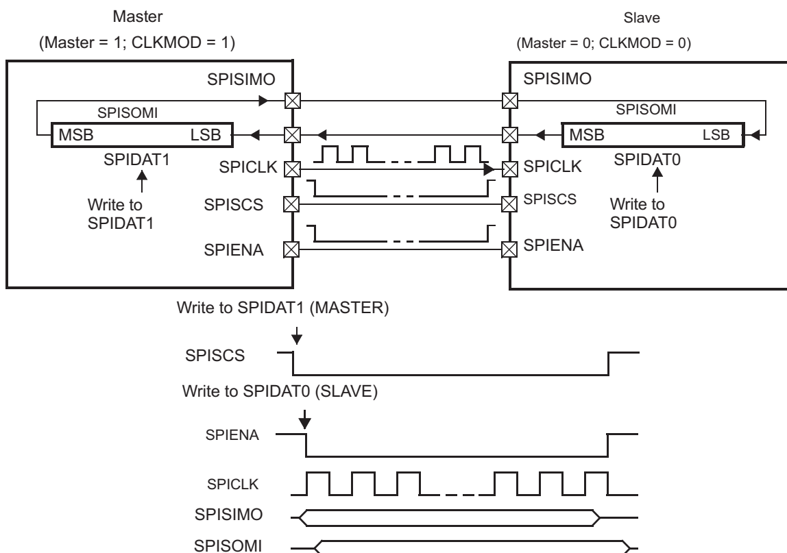
Figure 21-5. SPI Five-Pin Option with \overline{\text{SPIENA}} and \overline{\text{SPISCS}}
