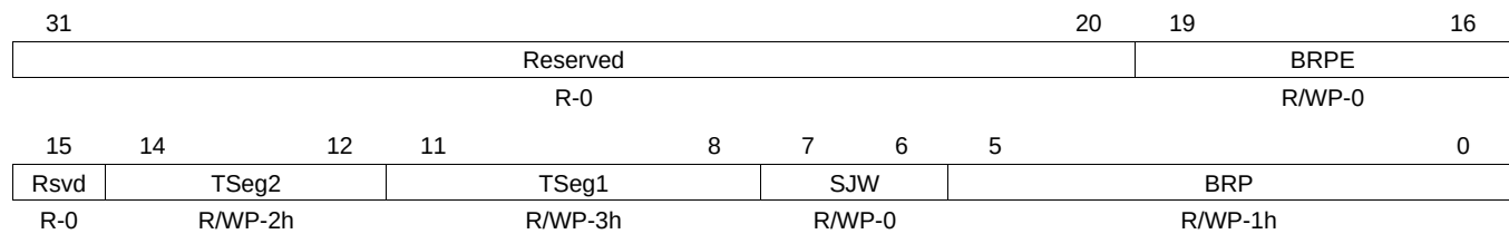
Figure 20-22. Bit Timing Register (DCAN BTR) [offset = 0Ch]
