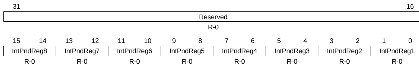
Figure 20-37. Interrupt Pending X Register (DCAN INTPND X) [offset = ACh]
