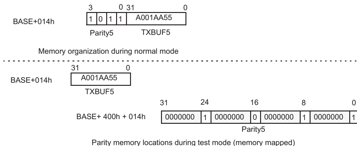
Figure 21-66. Example of Memory Mapped Parity Locations during Test Mode
