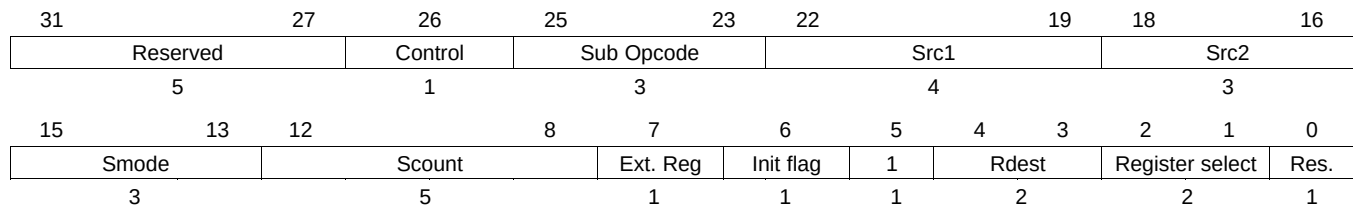
Figure 17-79. ADC, ADD, AND, OR, SBB, SUB, XOR Control Field (C31:C0)
