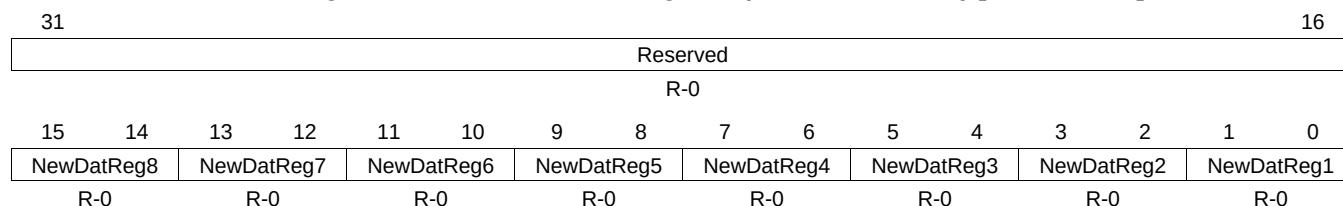
Figure 20-32. New Data X Register (DCAN NWDAT X) [offset = 98h]
