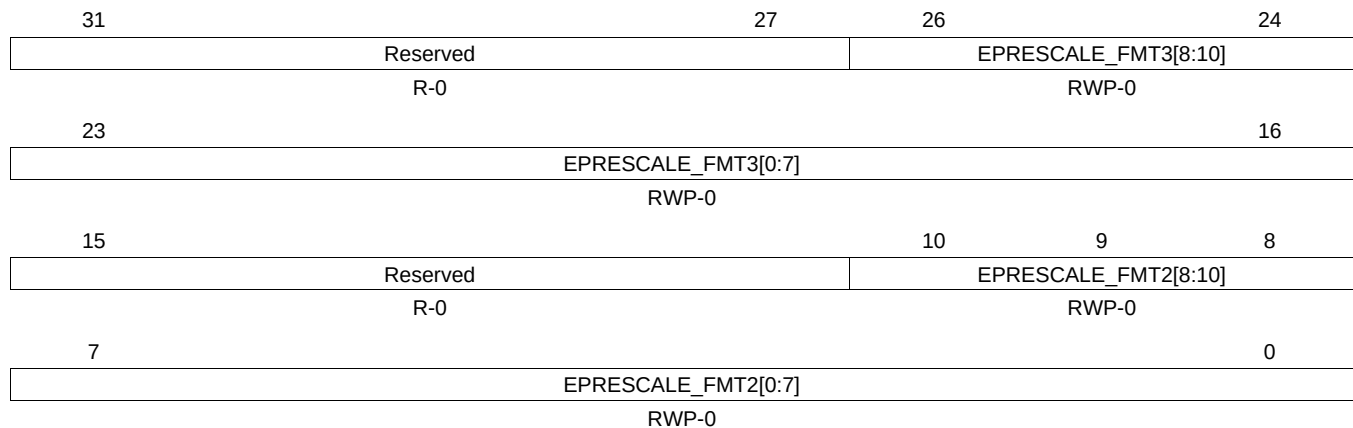
Figure 21-61. SPI Extended Prescale Register 2 (EXTENDED_PRESCALE2 for SPIFMT2 and SPIFMT3) [offset = 13Ch]
