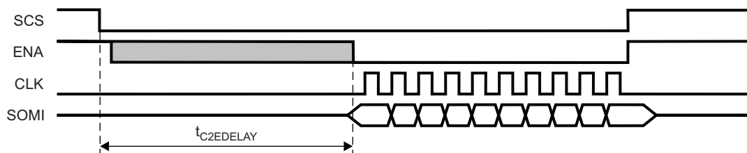
Figure 21-39. Chip-Select-Active-to-ENA-Signal-Active-Timeout
