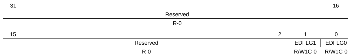
Figure 21-55. Multi-buffer RAM Uncorrectable Parity Error Status Register (UERRSTAT) [offset = 124h]
