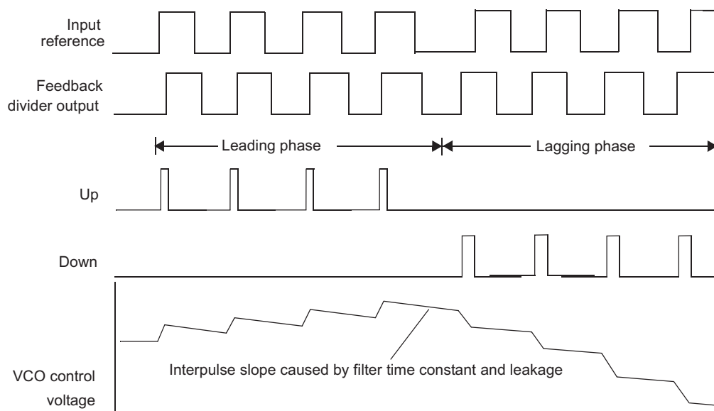
Figure 9-10. PFD Timing
