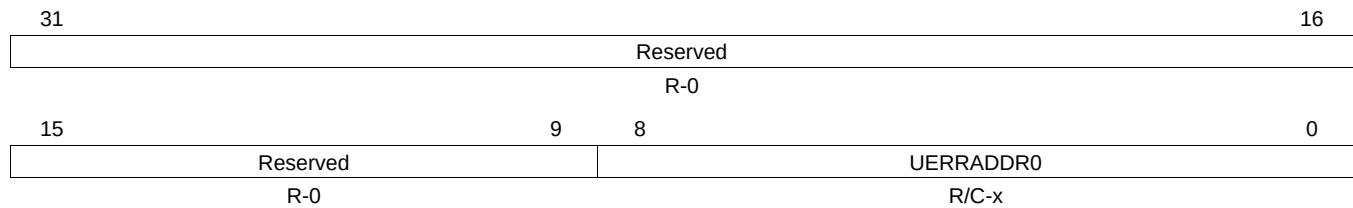
Figure 21-57. TXRAM Uncorrectable Parity Error Address Register (UERRADDR0) [offset = 12Ch]
