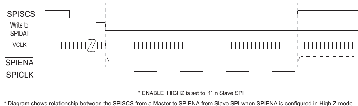
Figure 21-74. SPI/MibSPI Pins During Slave Mode in 5-pin Configuration - (Single/Multi Slave)
