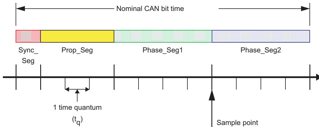
Figure 20-2. Bit Timing
