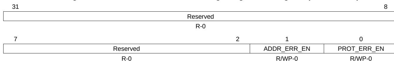
Figure 3-9. ERR_ENABLE_REG: Error Signaling Enable Register (Offset = E8h)
