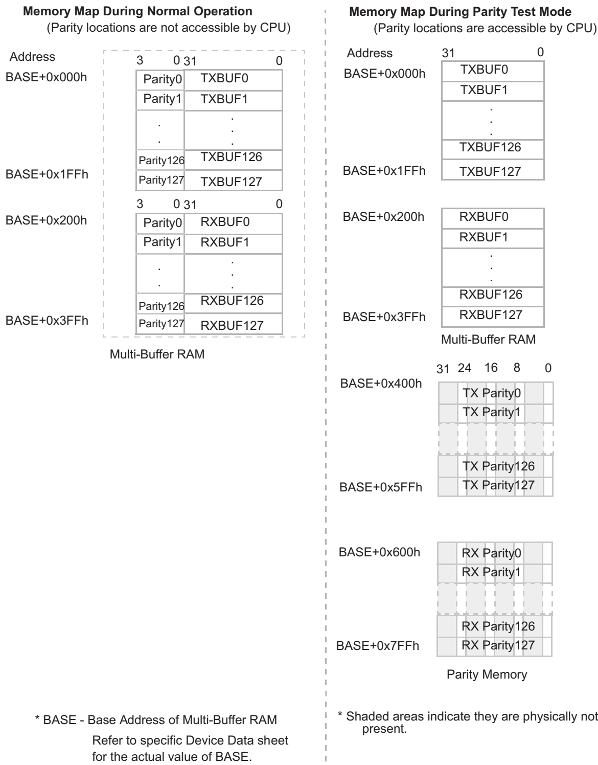
Figure 21-65. Memory Map for Parity Locations during Normal and Test Mode
