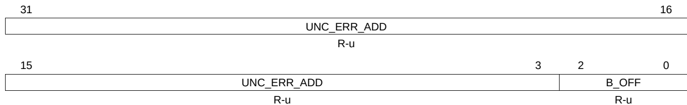
Figure 4-15. Flash Uncorrectable Error Address Register (FUNC_ERR_ADD) [offset = 20h]
