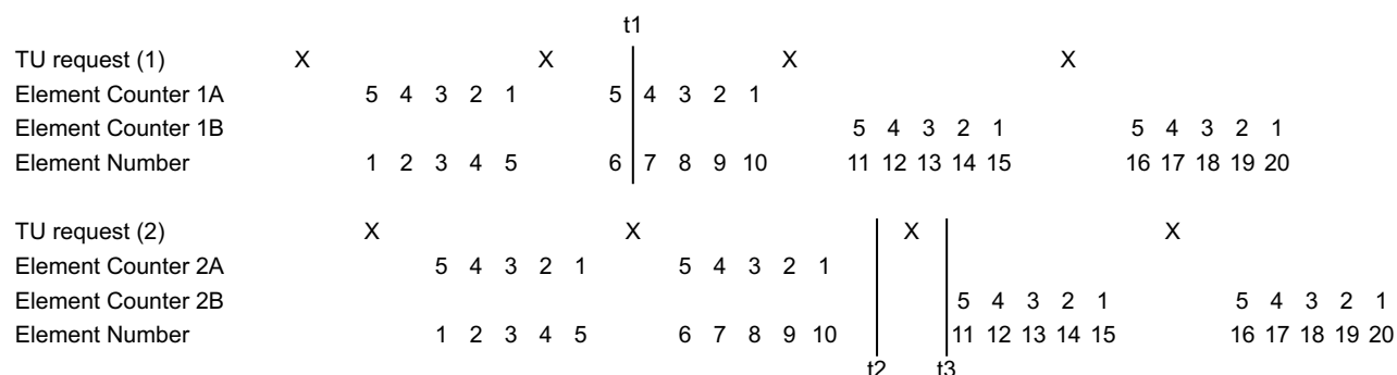
Figure 18-6. Dual Buffer Timing
