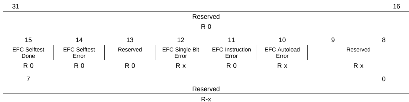
Figure 23-3. EFC Pins Register (EFCPINS) [offset = 2Ch]
