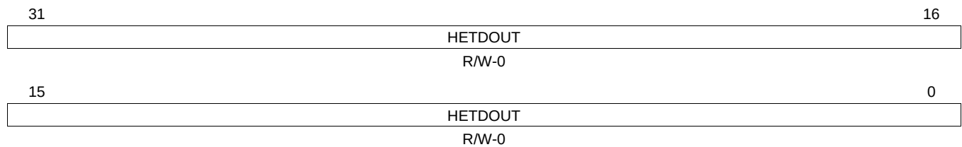
Figure 17-53. N2HET Data Output Register (HETDOUT) [offset = 54h]
