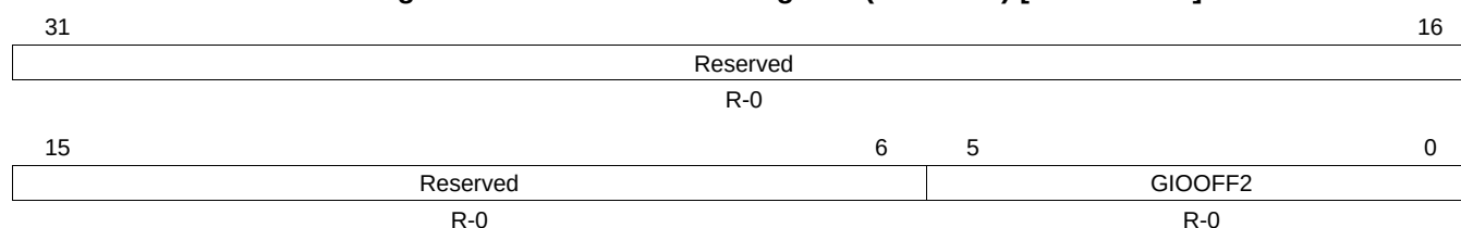
Figure 19-14. GIO Offset 2 Register (GIOFF2) [offset = 28h]
