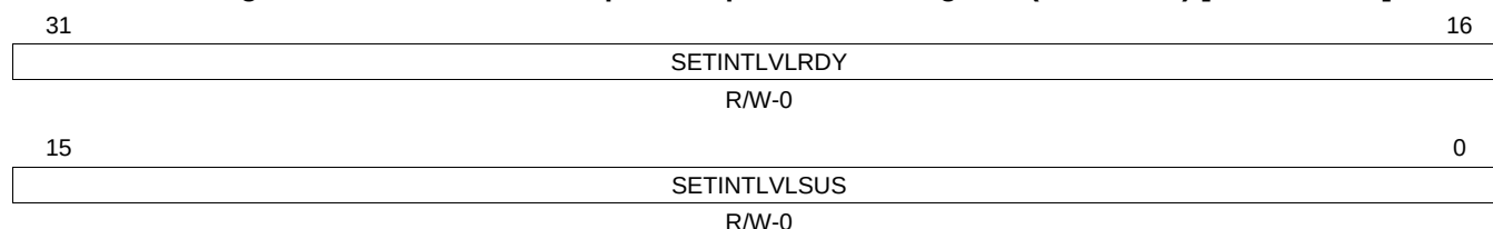
Figure 21-47. Transfer Group Interrupt Level Set Register (TGITLVST) [offset = 7Ch]
