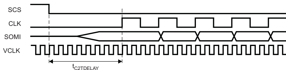
Figure 21-36. Example: t_{C2TDELAY} = 8 VCLK Cycles
