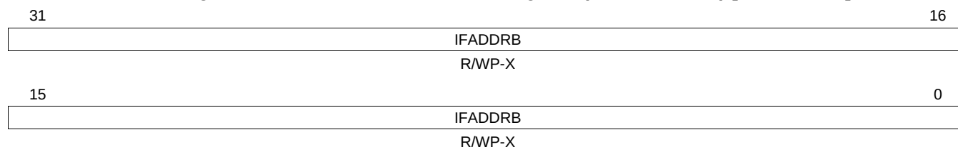
Figure 18-43. Initial Full Address B Register (HTU IFADDRB) [offset = 04h]
