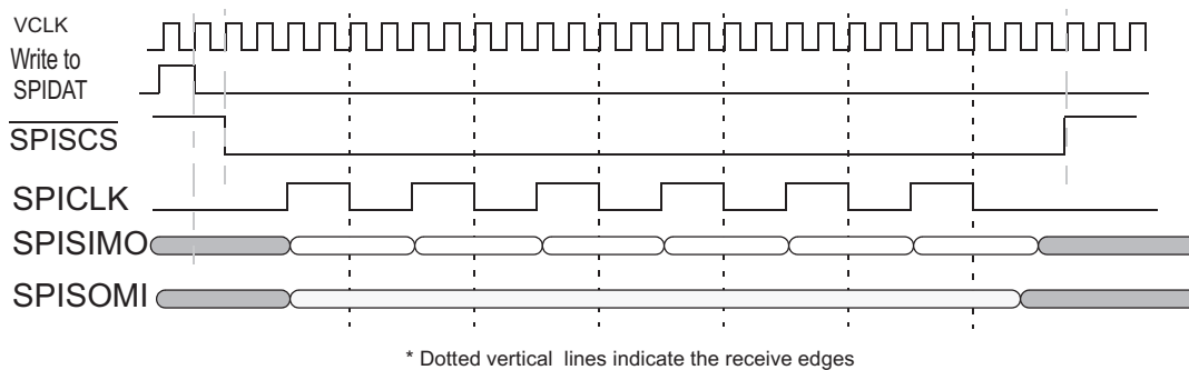
Figure 21-68. SPI/MibSPI Pins During Master Mode 4-pin with \overline{\text{SPISCS}} Configuration
