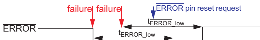
Figure 11-7. \overline{\text{ERROR}} Pin Timing - Example 4
