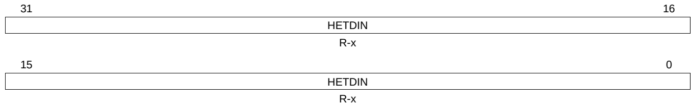
Figure 17-52. N2HET Data Input Register (HETDIN) [offset = 50h]
