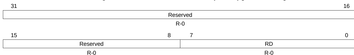
Figure 22-40. Receiver Data Buffer (SCIRD) [offset = 34h]
