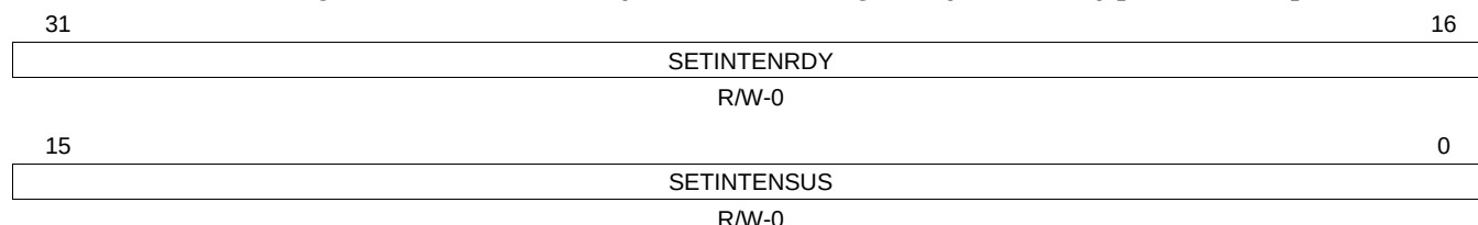
Figure 21-45. TG Interrupt Enable Set Register (TGITENST) [offset = 74h]
