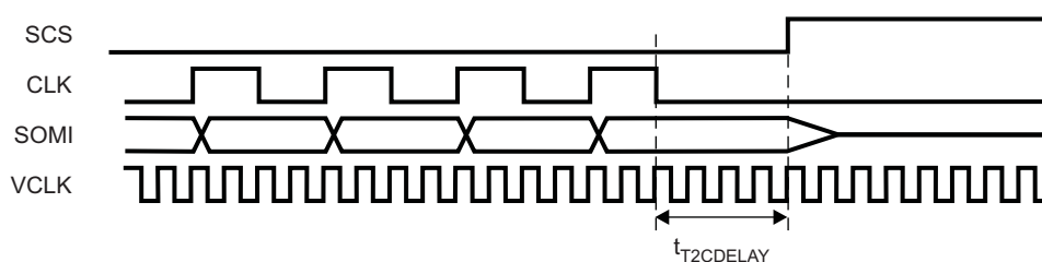
Figure 21-37. Example: t_{T2CDELAY} = 4 VCLK Cycles
