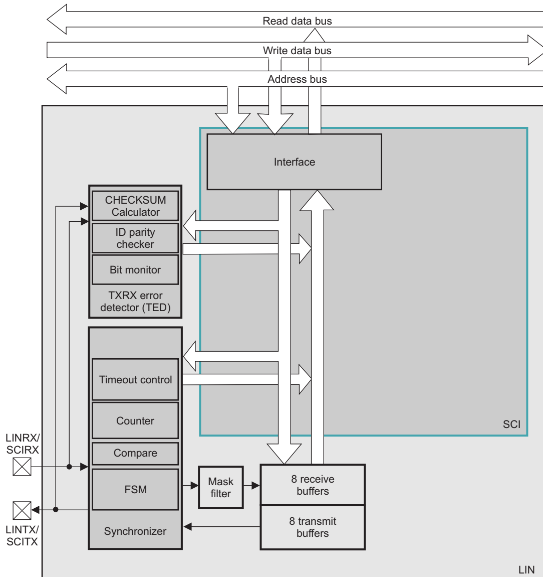
Figure 22-2. SCI/LIN Block Diagram
