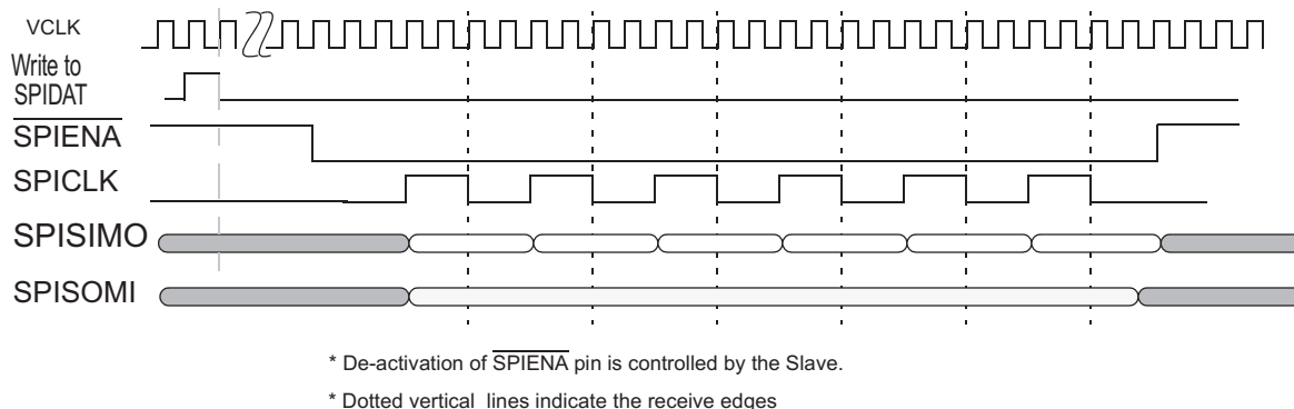
Figure 21-69. SPI/MibSPI Pins During Master Mode in 4-pin with \overline{\text{SPIENA}} Configuration
