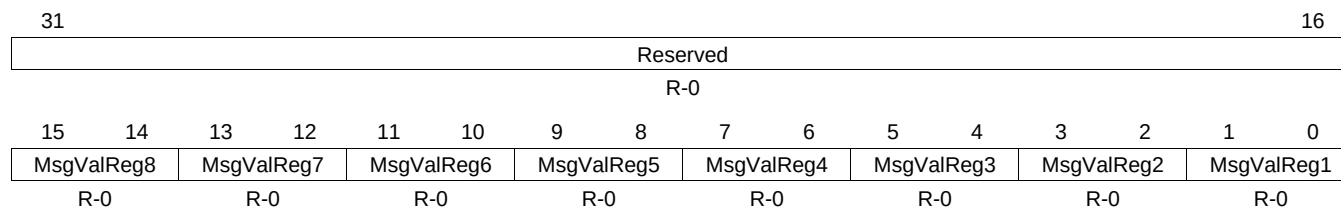
Figure 20-42. Message Valid X Register (DCAN MSGVAL X) [offset = C0h]
