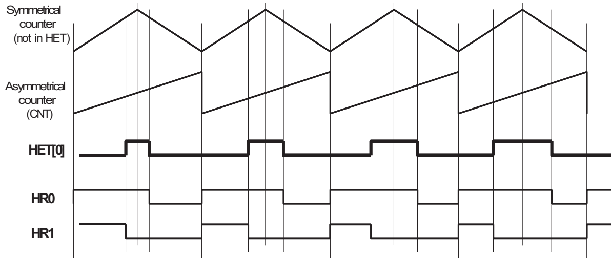
Figure 17-14. Symmetrical PWM with XOR-sharing Output
