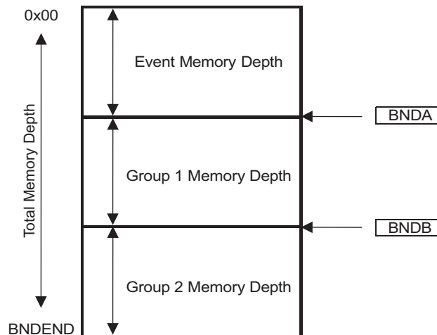
Figure 16-2. FIFO Implementation
