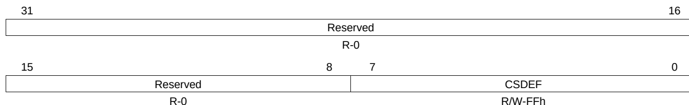
Figure 21-40. SPI Default Chip Select Register (SPIDEF) [offset = 4Ch]
