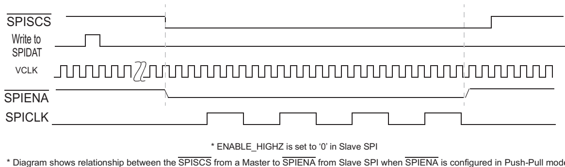
Figure 21-73. SPI/MibSPI Pins During Slave Mode in 5-pin Configuration - (Single Slave)
