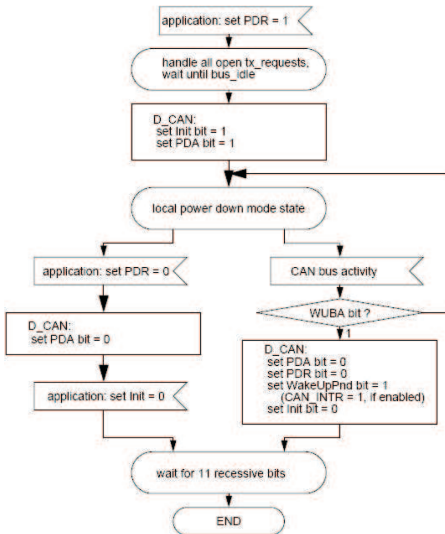
Figure 20-14. Local Power-Down Mode Flow Diagram
