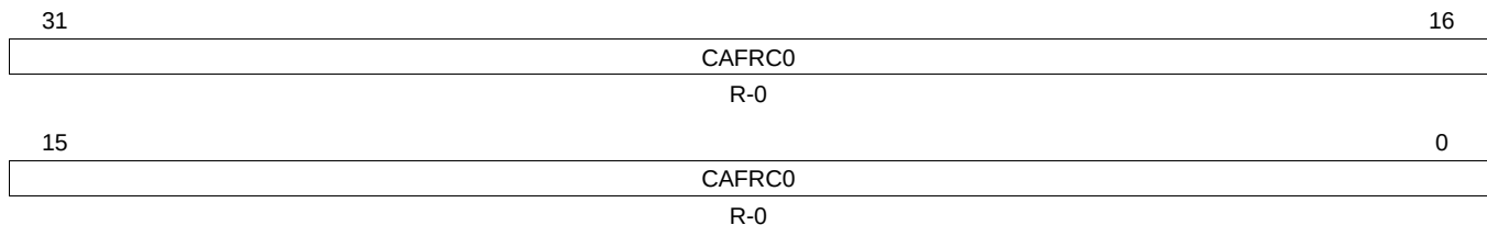
Figure 12-14. RTI Capture Free Running Counter 0 Register (RTICAFRC0) [offset = 20h]
