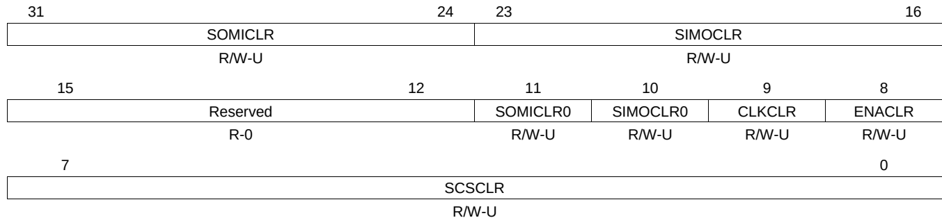
Figure 21-27. SPI Pin Control Register 5 (SPIPC5) [offset = 28h]
