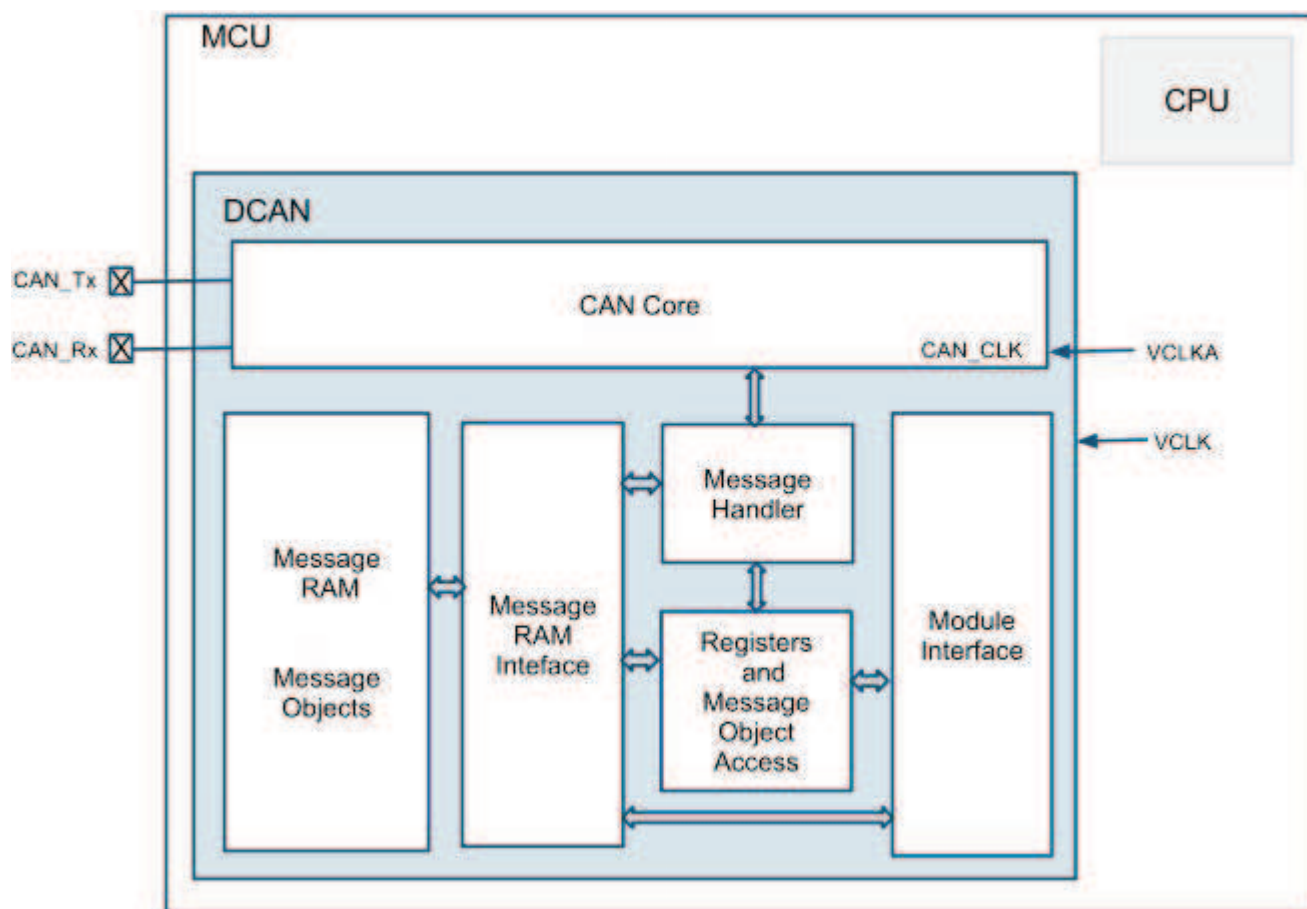
Figure 20-1. Block Diagram
